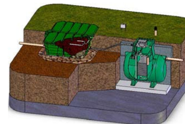
Above: Puraflo Tertiary Treatment Option: capable of achieving a 5:5 BOD/TSS standard.
