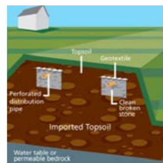
Section Through Raised Mounded Percolation Area
