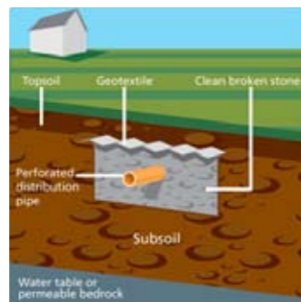
Section Through Normal Percolation Area
